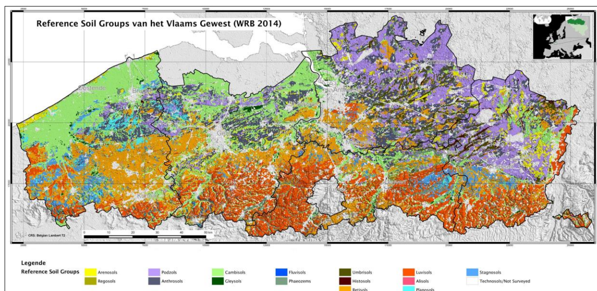
Figure AI.1. Soil map of Flanders 1:250 000 - urban areas (Technosols) in white based on city limits
