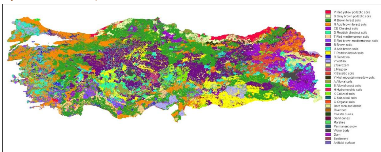
Figure 3.4. Soils of Türkiye and miscellaneous units
