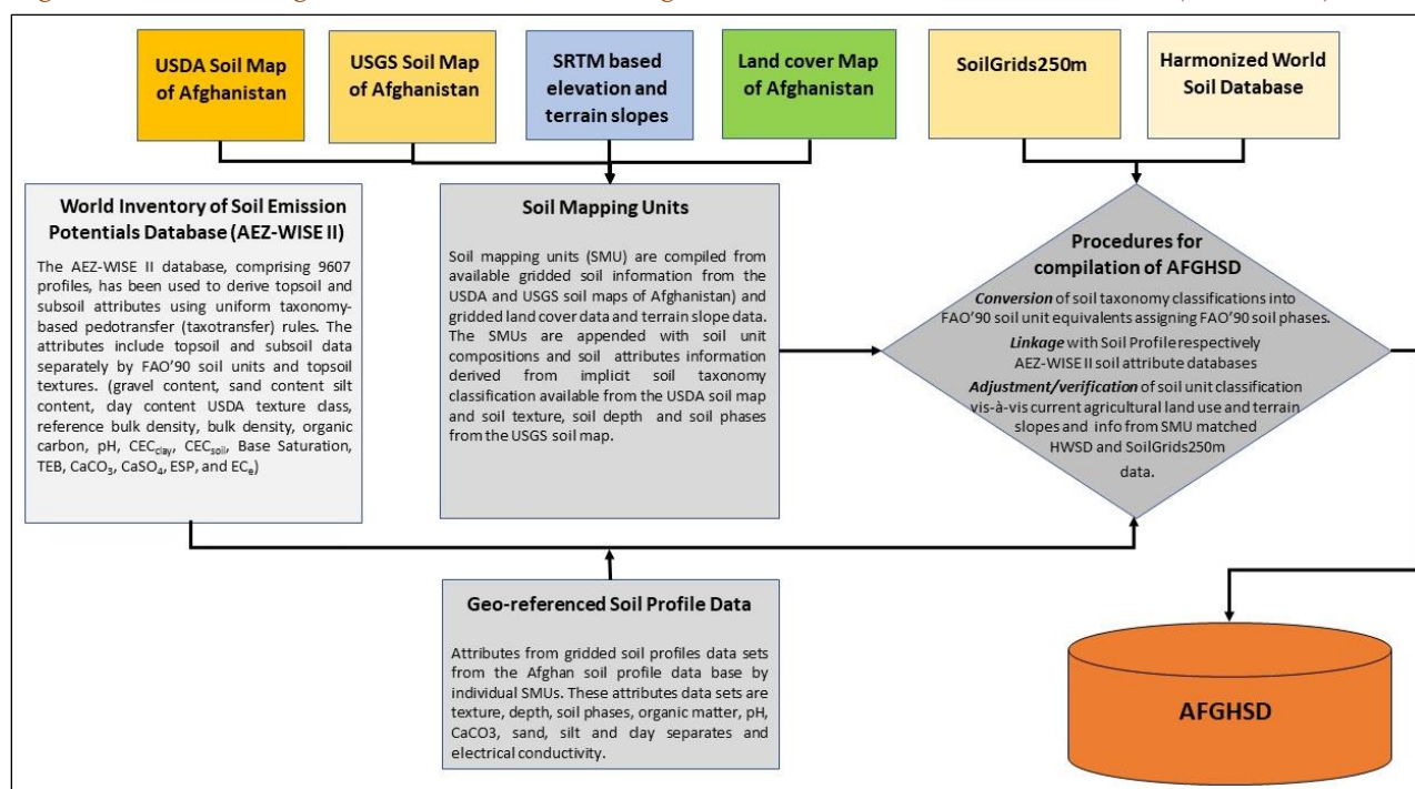
Figure 3.1. Data integration for the National Afghanistan Harmonized Soil Database (AFGHSD)
