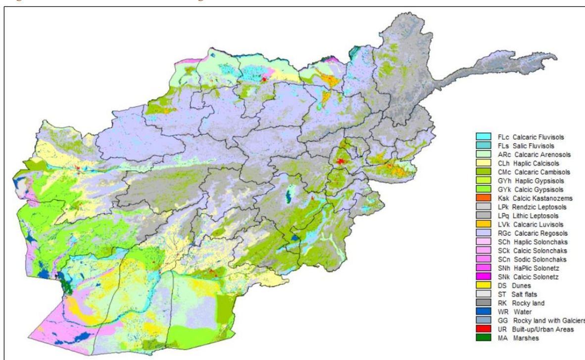
Figure 3.2. Dominant soils of Afghanistan
