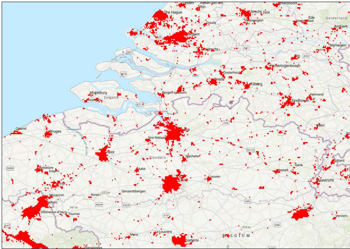
Figure AI.2. Map of Flanders extracted from HWSD v2.0 viewer urban areas (Technosols) in red, based on WorldCover 2020 (built-up class with 50% threshold)
