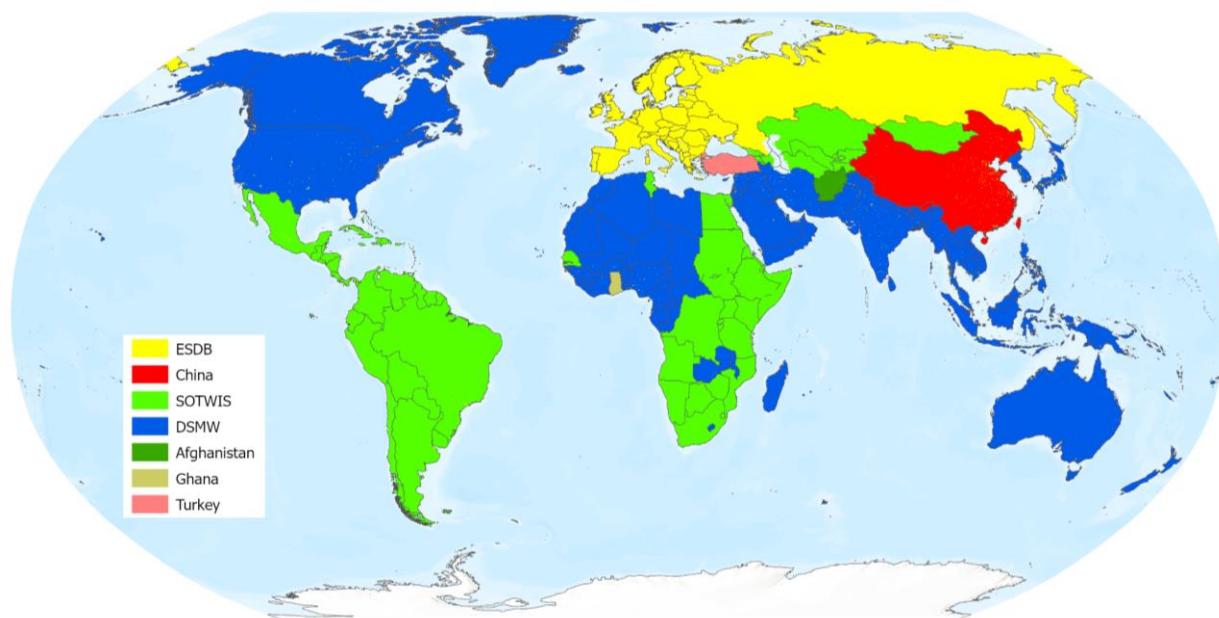
Figure 3.5. Source areas and countries in HWSD v2.0
