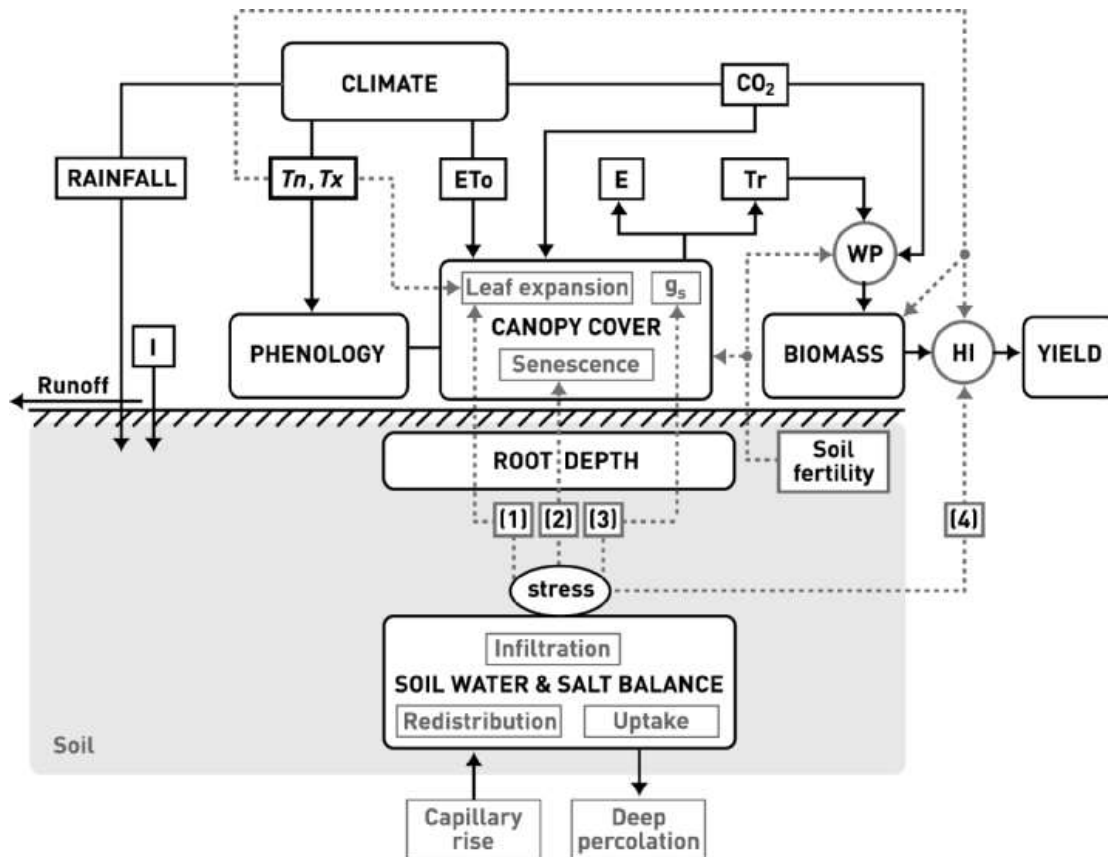
Figure 1.1b – Chart of AquaCrop indicating the main components of the soil–plant–atmosphere continuum and the parameters driving phenology, canopy cover, transpiration, biomass production, and final yield. [I, irrigation; T_n , minimum air temperature; T_x , maximum air temperature; ET_o , reference evapotranspiration; E, soil evaporation; Tr , canopy transpiration; g_s , stomatal conductance; WP, water productivity; HI, harvest index; CO_2 , atmospheric carbon dioxide concentration; (1), (2), (3), (4), water stress response functions for leaf expansion, senescence, stomatal conductance and harvest index, respectively]. Continuous lines indicate direct links between variables and processes. Dashed lines indicate feedbacks. See section 1.2 for a more extensive description.
