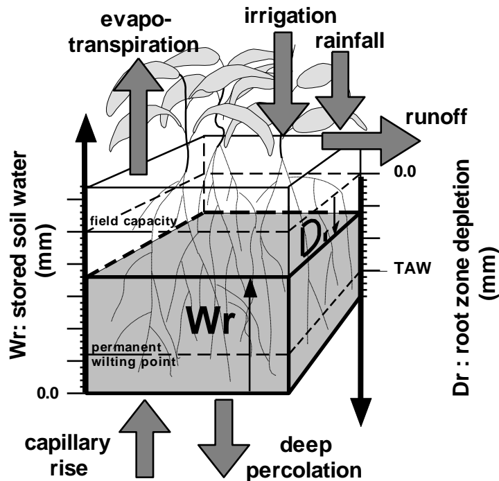
Figure 1.2b – The root zone as a reservoir with indication of the fluxes at its boundaries affecting the water stored in the root zone ( W_r ) and the root zone depletion ( D_r )
