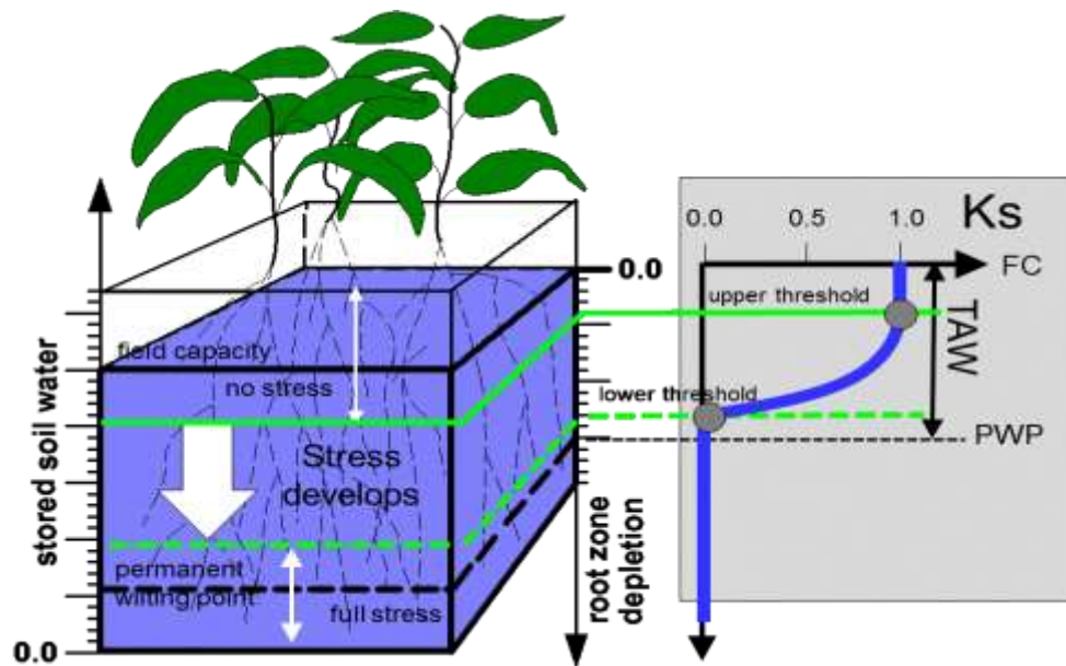
Figure 1.2c – The water stress coefficient ( K_s ) for various degrees of root zone depletion ( D_r ). TAW is the Total Available soil Water in the root zone which is the difference between the water content at Field Capacity and Permanent Wilting Point
