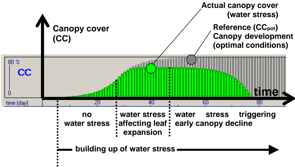
Figure 1.2e – Simulation of the green canopy cover (CC) when water stress builds during the crop cycle with reference to the canopy development for non stressed conditions ( CC_{pot} )
