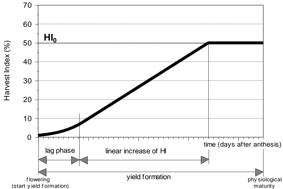
Figure 1.2j – Building up of Harvest Index from flowering till physiological maturity for fruit and grain producing crops
