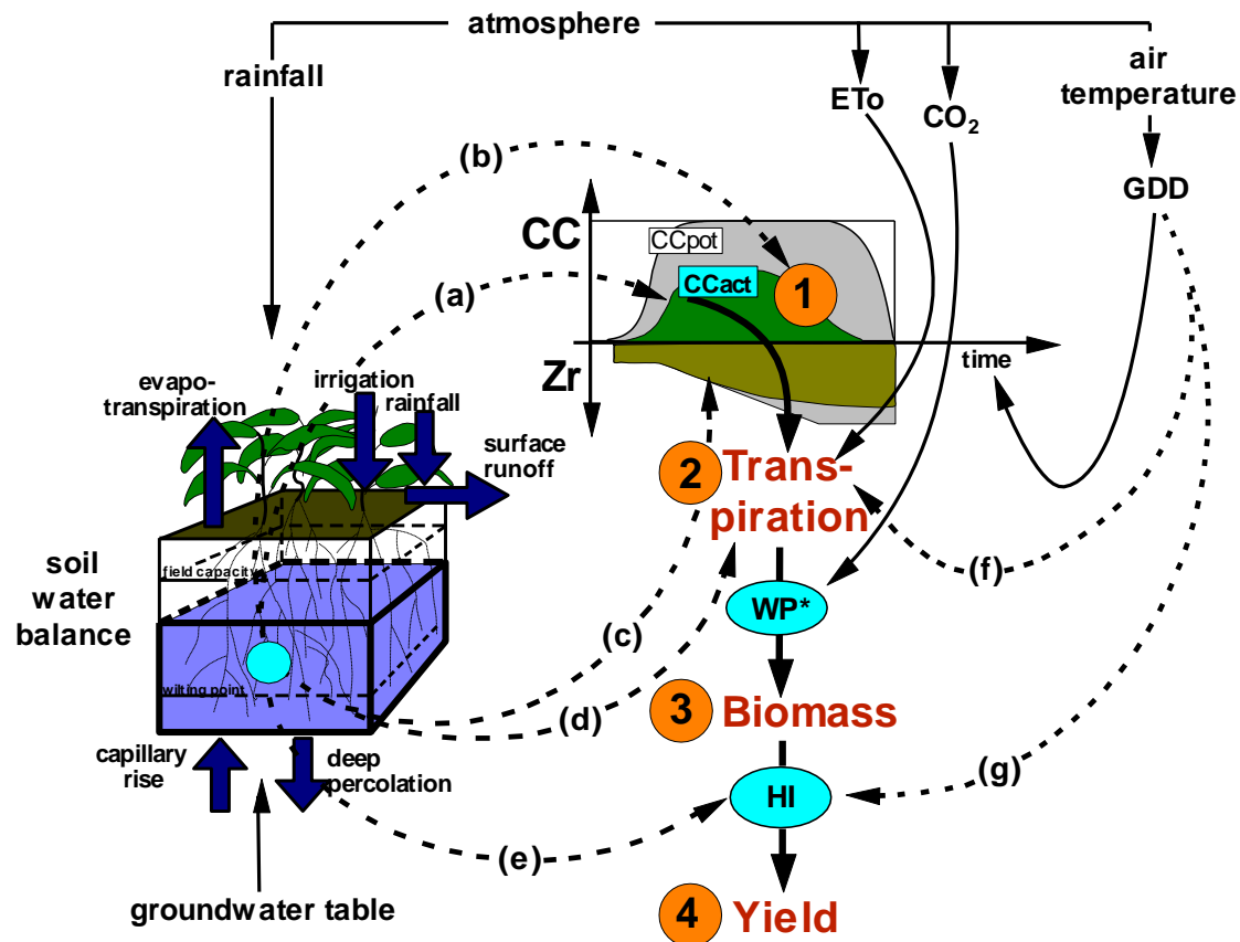
Figure 1.2a – Calculation scheme of AquaCrop with indication (dotted arrows) of the processes affected by water stress (a to e) and temperature stress (f to g). CC is the simulated canopy cover, CC pot the potential canopy cover, Z r the rooting depth, ETo the reference evapotranspiration, GDD the growing degree days, WP* the normalized crop water productivity, and HI the Harvest Index.
