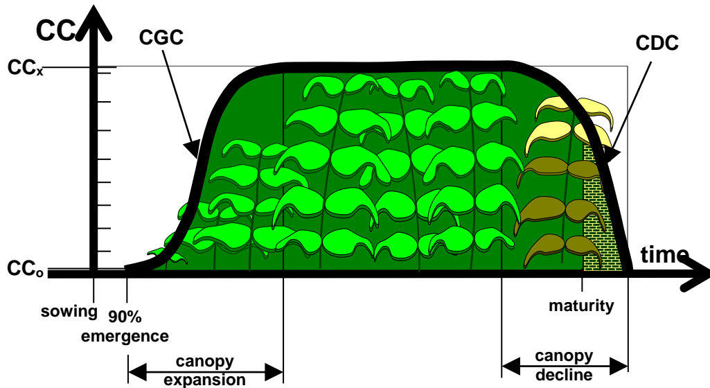
Figure 1.2d – Variation of the green canopy cover (CC) throughout the crop cycle under non-stress conditions. CC_0 and CC_x are the initial and maximum green canopy cover, respectively; CGC is the green canopy growth coefficient; CDC is the green canopy decline coefficient
