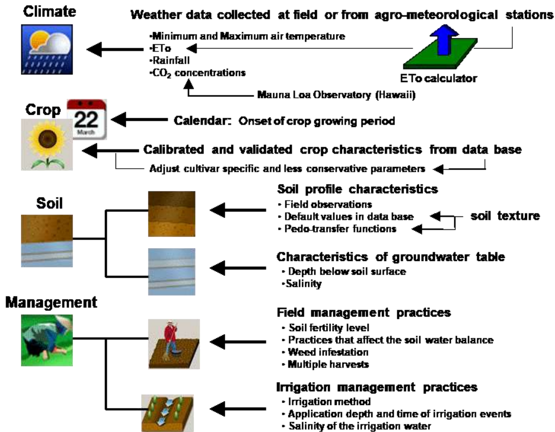
Figure 1.3 – Input data defining the environment in which the crop develops
