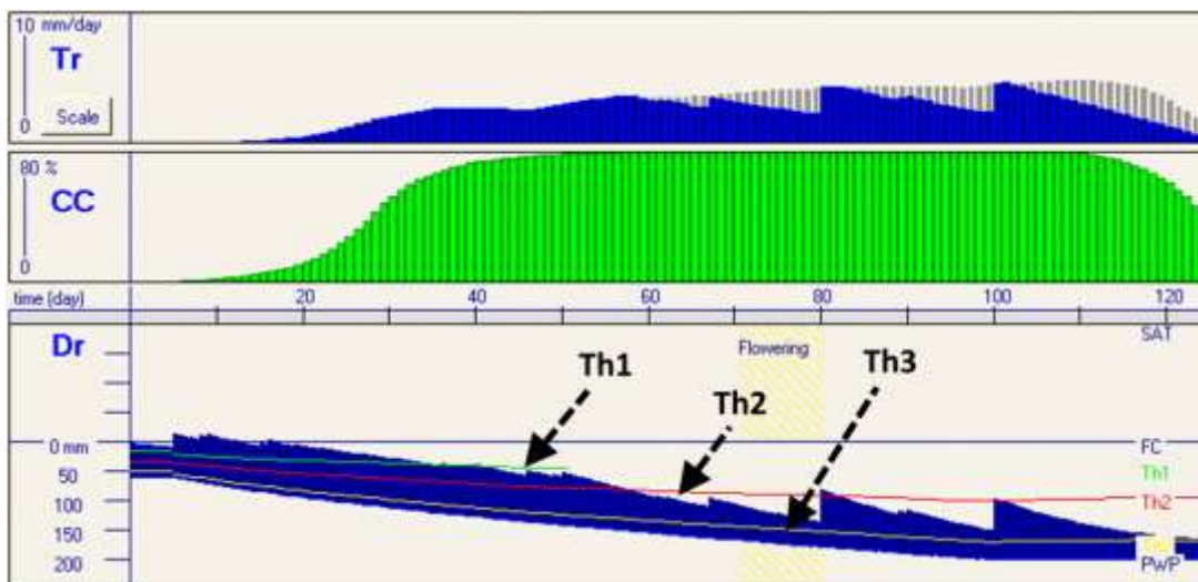
Figure 1.2g – Simulated root zone depletion (Dr), green canopy cover (CC) and crop transpiration (Tr) throughout the crop cycle with indication of the soil water thresholds affecting canopy development (Th1), inducing stomata closure (Th2), and triggering early canopy senescence (Th3)
