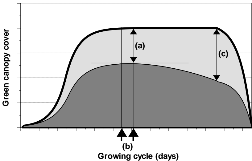
Figure 1.2f – Green canopy cover (CC) for unlimited (light shaded area) and limited (dark shaded area) soil fertility with indication of the processes resulting in (a) a less dense canopy cover, (b) a slower canopy development, and (c) a steady decline of CC once the maximum canopy cover is reached
