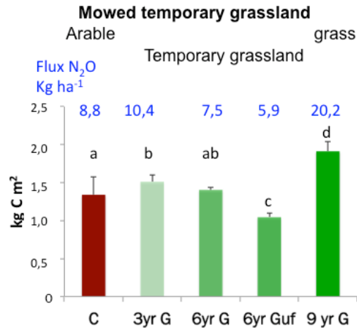
Fig. 1: Carbon storage in soils from the study site, including 9 years continuous crop (C), 9 years continuous grassland (9yrG), and temporary grasslands after 3 years of crop, which include 3 years fertilized grassland (3yrG), 6 years fertilized grassland (6yrG) and 6 years of unfertilized grassland (6yrGuf)
