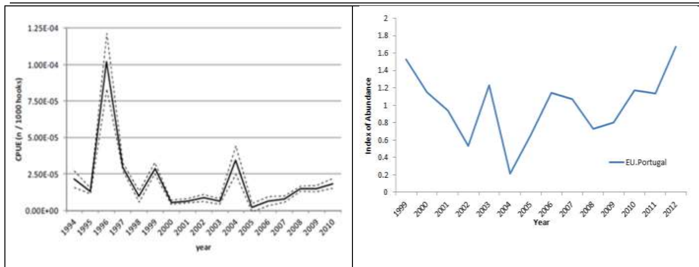
Fig. 2. Shortfin mako shark: Standardised longline CPUE series for shortfin mako shark in the Indian Ocean for the Japanese fleet (1994–2010) (left) and the EU, Portugal fleets (1999–2012) (right).
