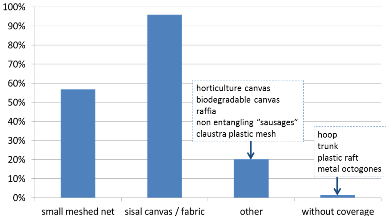
Figure 4: types of FAD coverage used by the ANABAC/OPAGAC skippers
