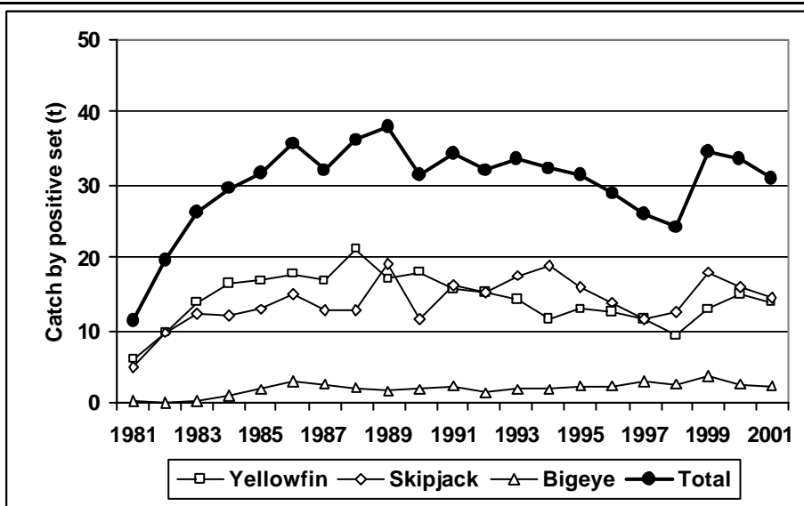
Figure 4 : Catches per unit of effort (tons by positive set) according to the fishing mode
