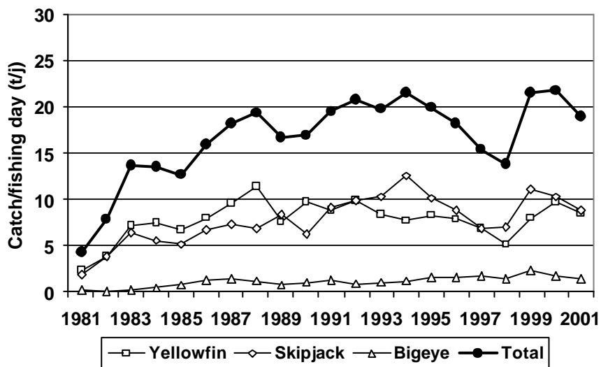
Figure 3 : Catches per unit of effort (tons by fishing day) according to the fishing mode
