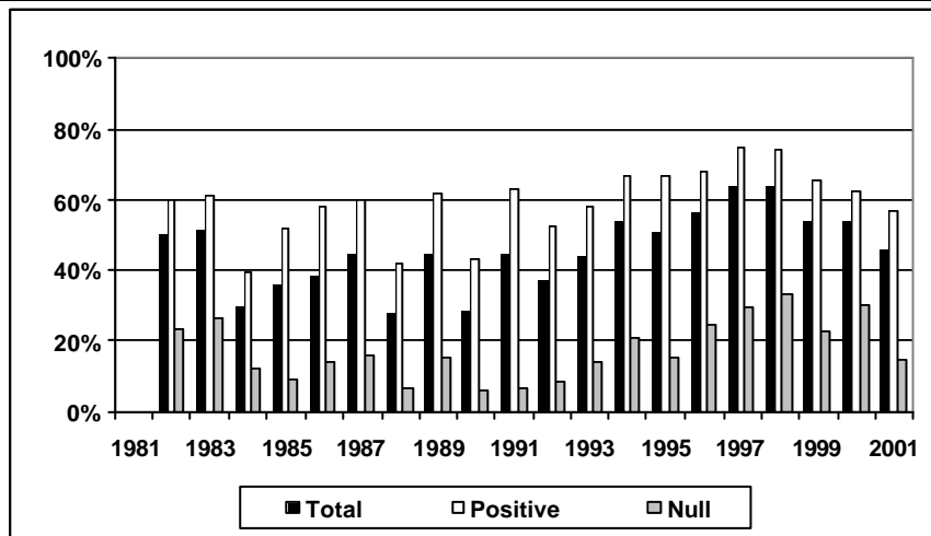
Figure 1: Fishing effort of the French fleet : Purse seiners number according to their GRT category (1 a), Number of one degree squares visited according to different levels of effort (1 b), Carrying capacity, fishing and searching days (1 c), Percentage of log sets (1 d)
