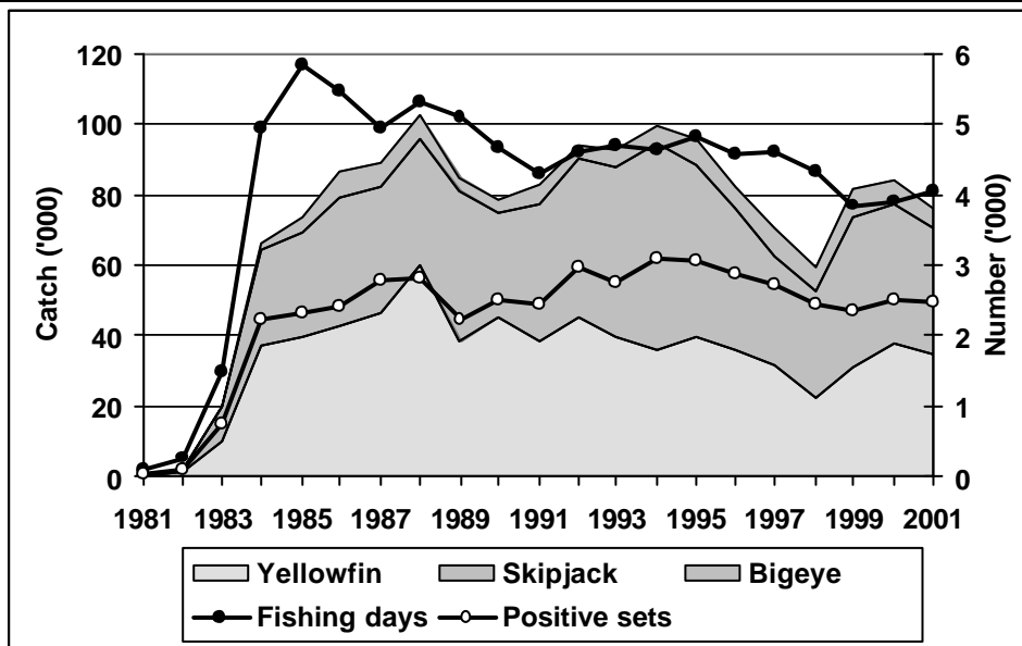
Figure 2 : Catches by species and fishing effort according to the fishing mode
