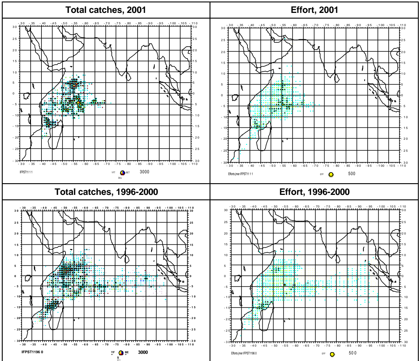
Figure 7: Spatial distribution of the French fleet total catches (left) and effort (right) in 2001 (above) and for the average situation over the period 1996-2000 (below)
