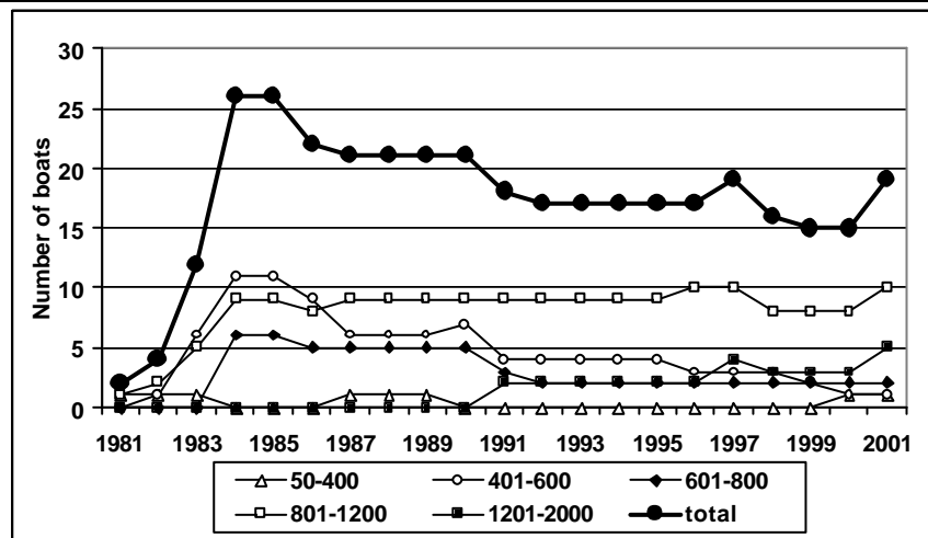
1 a – Purse seiners number according to their GRT category
