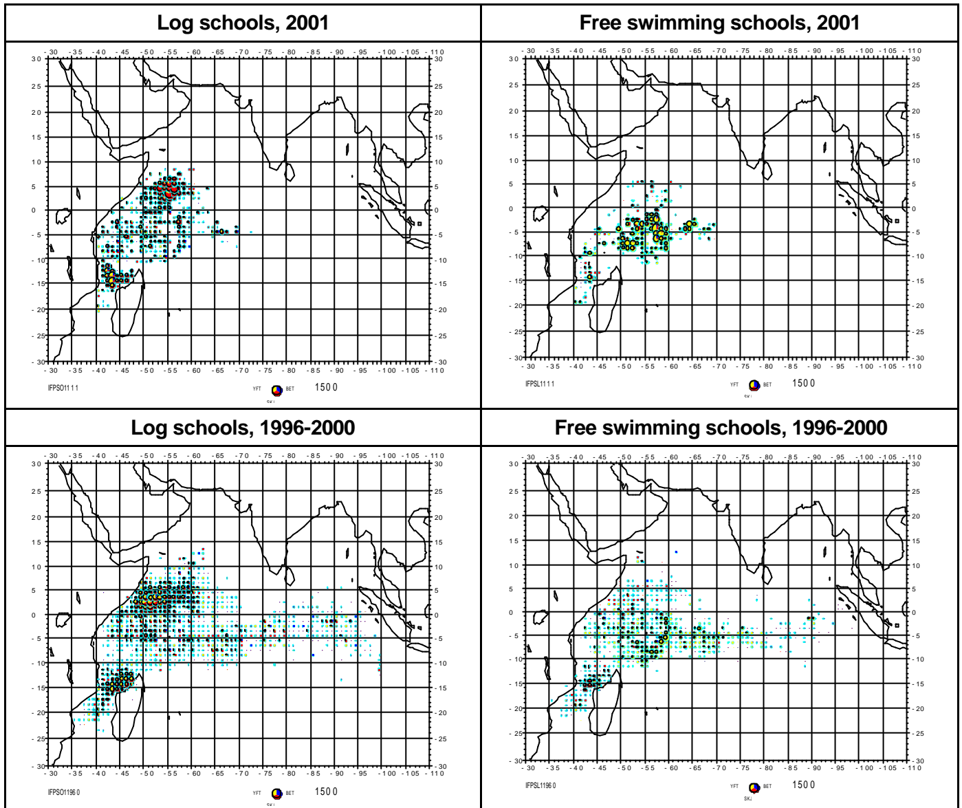
Figure 6: Spatial distribution of the French fleet catches by species according to the fishing mode (log schools, left and free swimming schools, right) in 2001 (above) and for the average situation over the period 1996-2000 (below)
