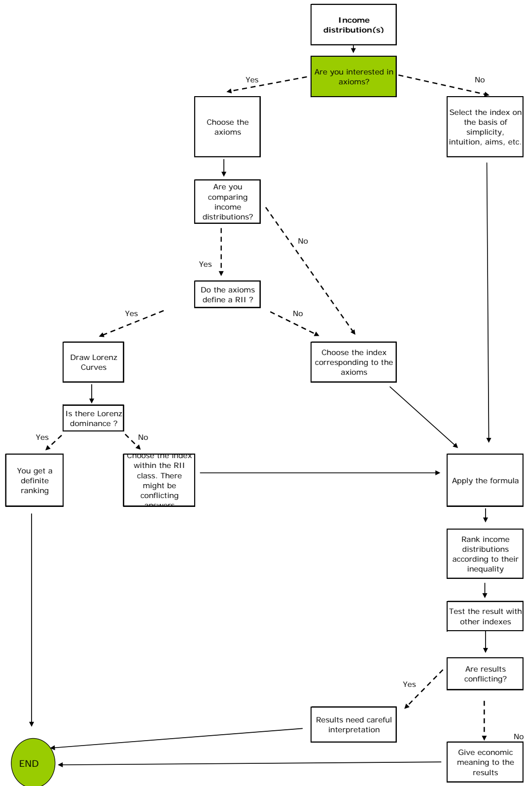
Figure 2: A general step-by-step procedure to choose inequality indexes
