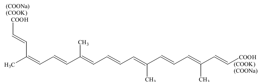
cis -Norbixin
