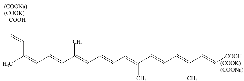
cis -Norbixin
